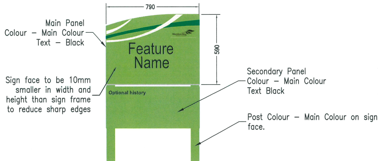
FRONT PANEL DETAIL
