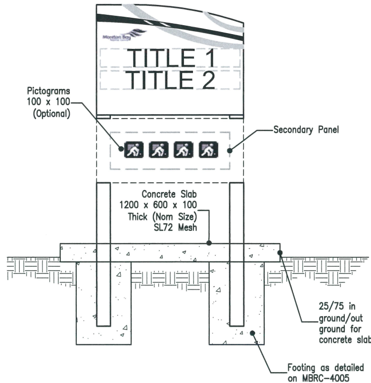
REAR ELEVATION (Optional)
