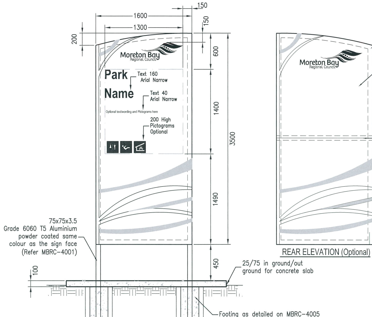
FRONT ELEVATION
