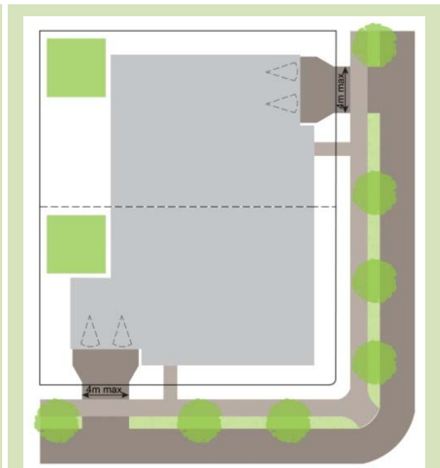
Example: Dual occupancy – corner lot separate driveways.
