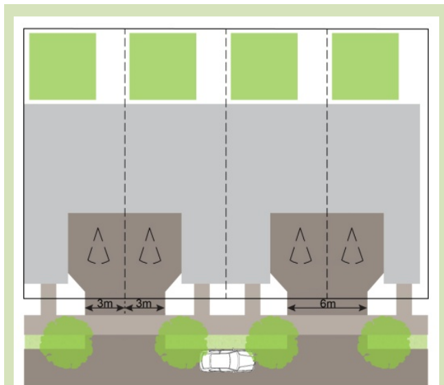
Example: individual driveways. 1.3m wide crossover per 7.5m of primary road frontage.
