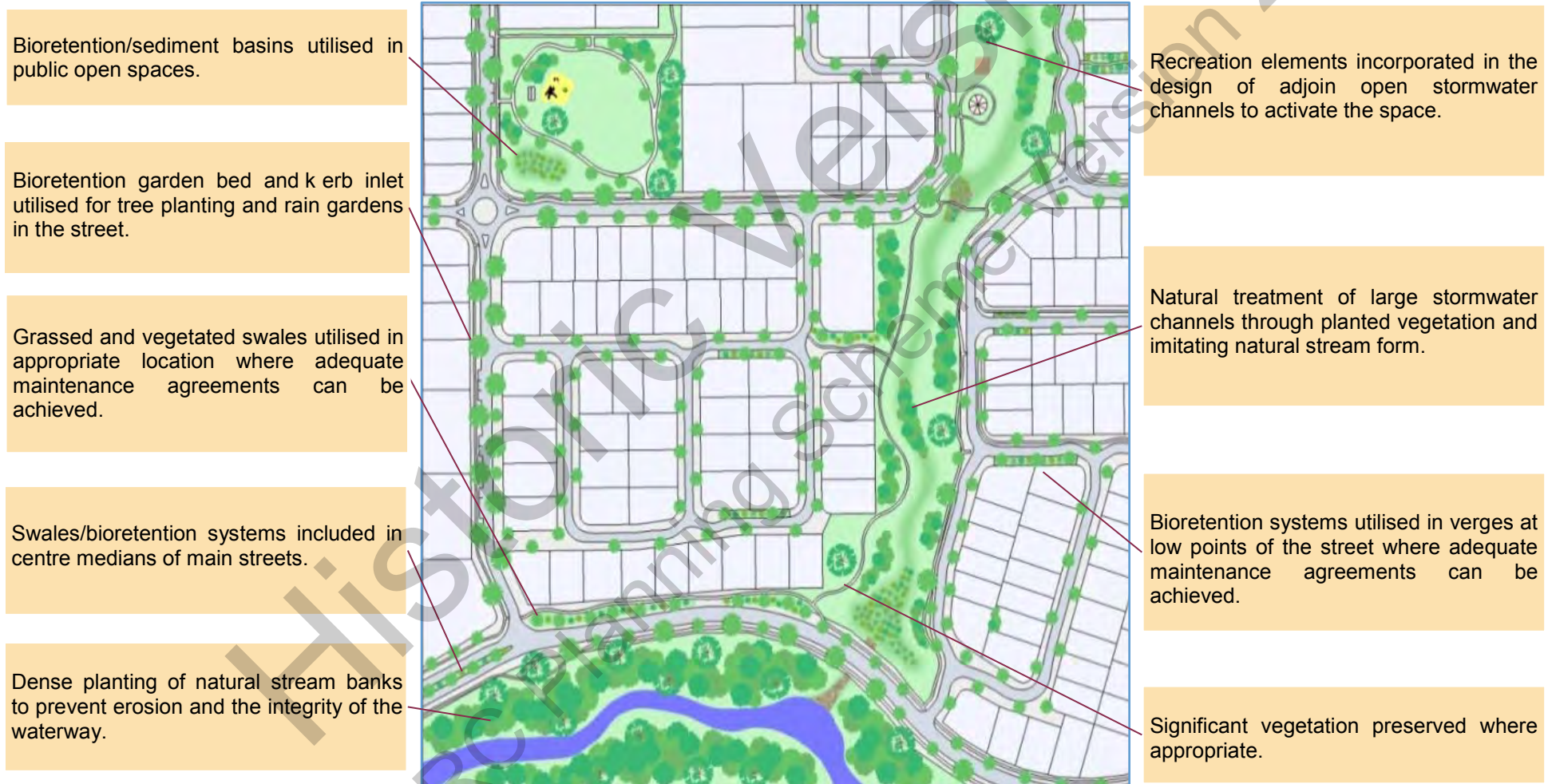
Figure 1.1: Indicative concept layout depicting possible locations for stormwater treatment in residential areas
