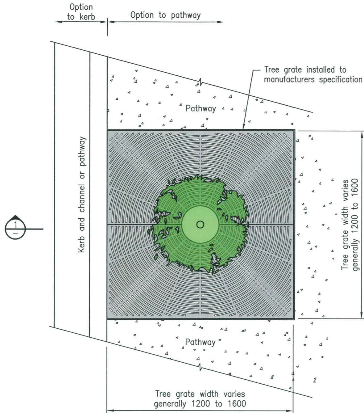
TREE GRATE PLAN Scale A
