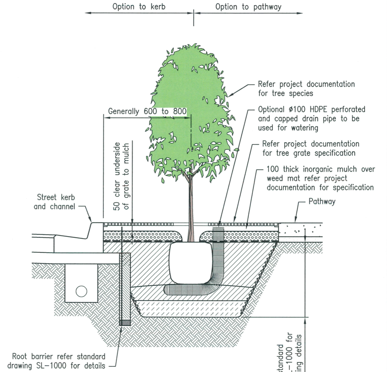
SECTION A Scale A
