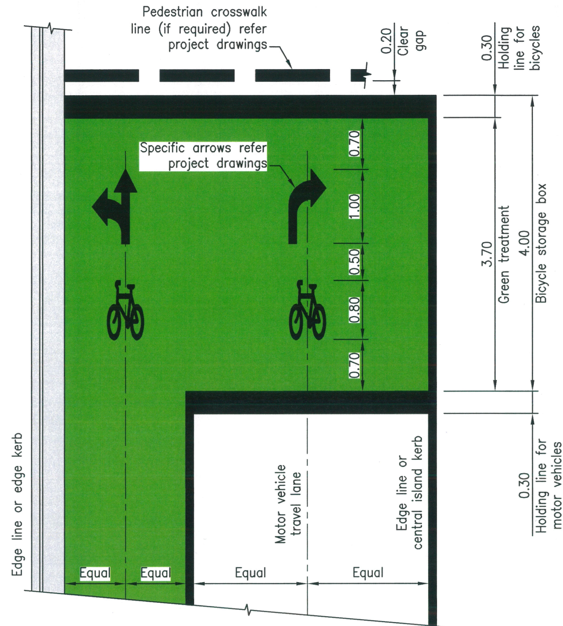
WITH CYCLIST TURNING PROVISION
