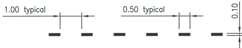
MODIFIED CONTINUITY LINE DETAIL
