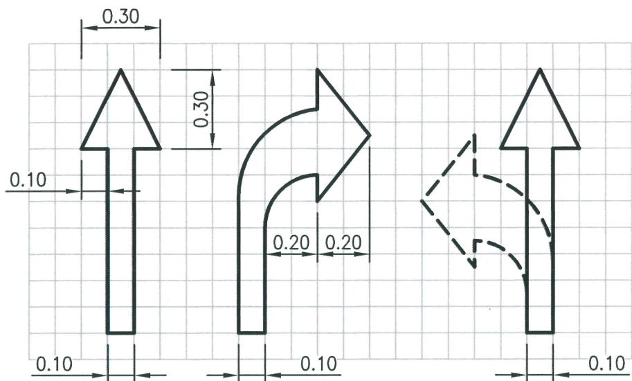
BICYCLE STORAGE BOX PAVEMENT ARROW DETAIL
