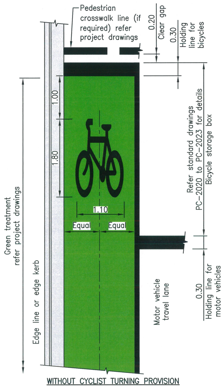
TYPICAL BICYCLE STORAGE BOX PAVEMENT MARKING PLAN
