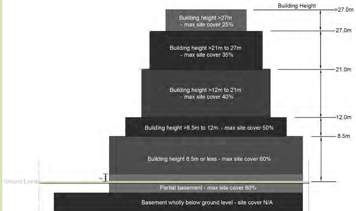
Site cover: Percentage vs Building height
