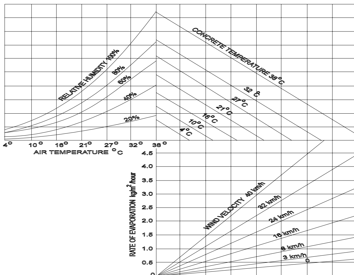
Figure C247.1 - Rate of Evaporation
