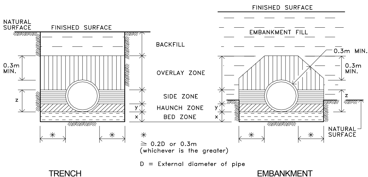
Figure C221.1 - Pipe Installation Conditions
