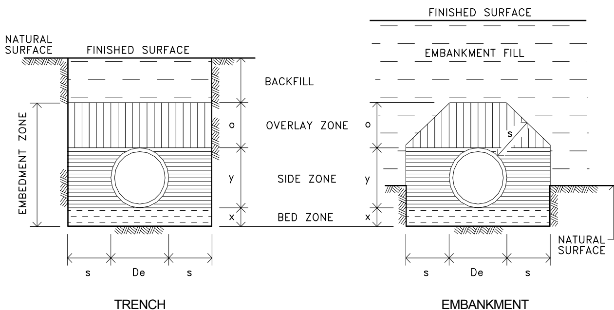
Figure C221.3 - PVC Pipe Installation Conditions
