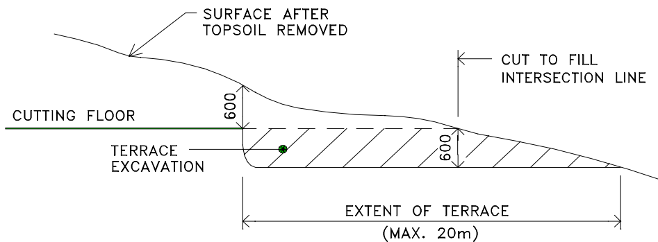
Figure C213.1 - Transition from Cut to Fill
