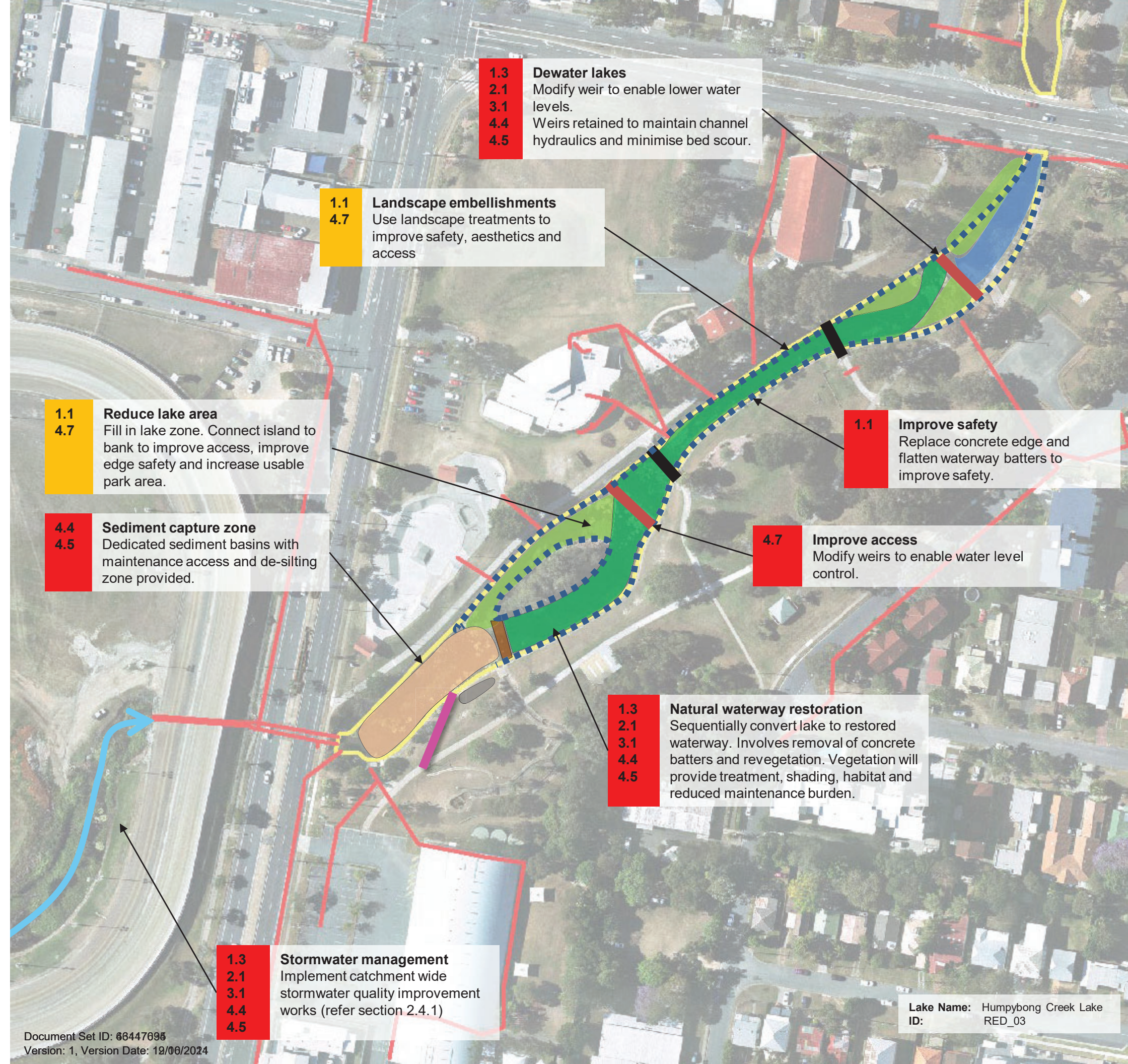
FIGURE 3-4: Rectification Concept Plan for Humpybong Creek RED_03 Lake
