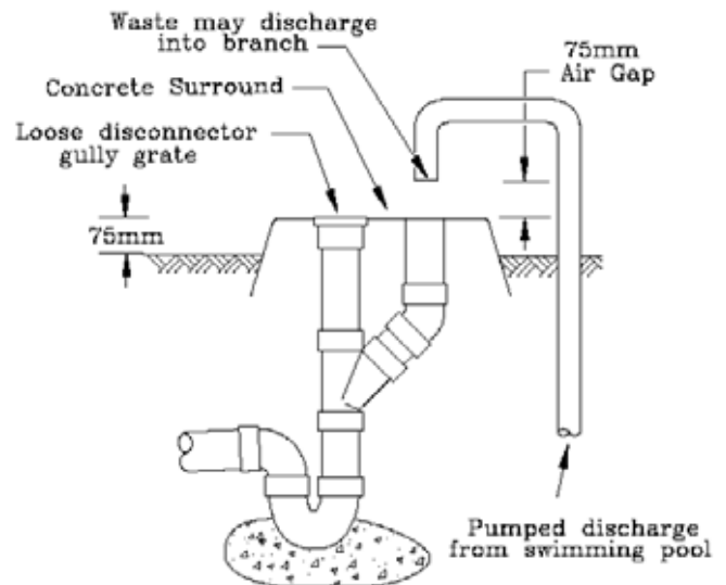
TYPICAL CONNECTION OF PUMPED WASTE DISCHARGE FROM SWIMMING POOLS
