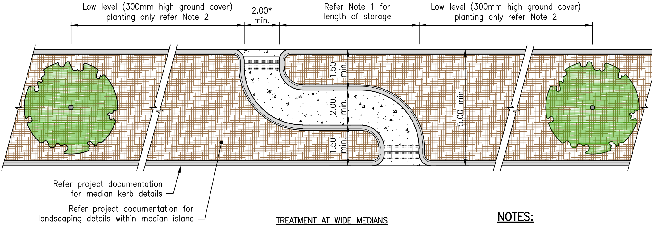
PLAN OF MEDIAN AT STAGED PEDESTRIAN CROSSING Scale A
